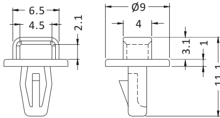
P.C.B Ø4.0 THICKNESS 1.6~2.0
