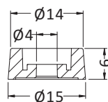
SECTION A-A FOOT
