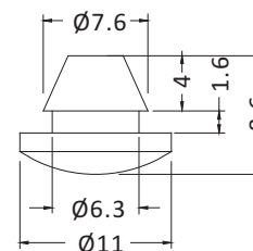
MOUNTING HOLE \varnothing 6.5
