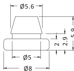
MOUNTING HOLE \varnothing 4.5~5.0 THICKNESS 0.8~1.0
