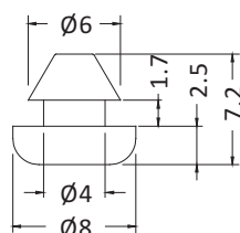
MOUNTING HOLE \varnothing 4.2
