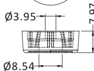
HOLE \varnothing 4.1 \sim \varnothing 4.2 THICKNESS 0.8~2.0
