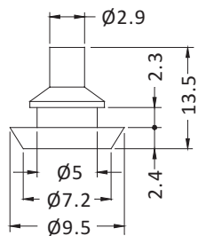
MOUNTING HOLE \varnothing 5.2
